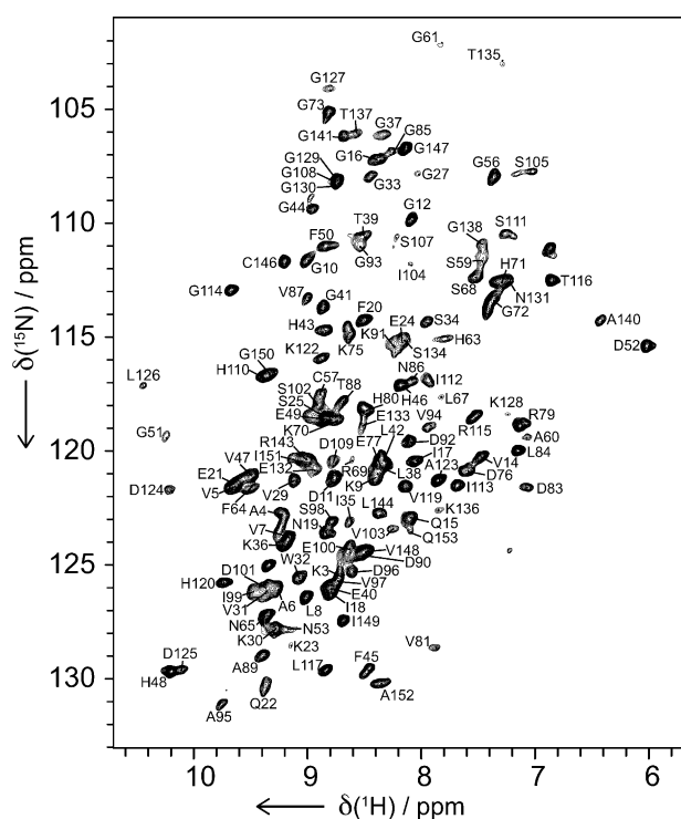
Figure 1. Assigned proton-detected HN correlation spectrum of human [100% ^1\text{H} , ^2\text{H} , ^{13}\text{C} , ^{15}\text{N} ]-Zn II -SOD at 1 GHz and 60 kHz MAS. Pulse sequences for all ^1\text{H} -detected correlations, as well as more experimental details, can be found in the Supporting Information.
