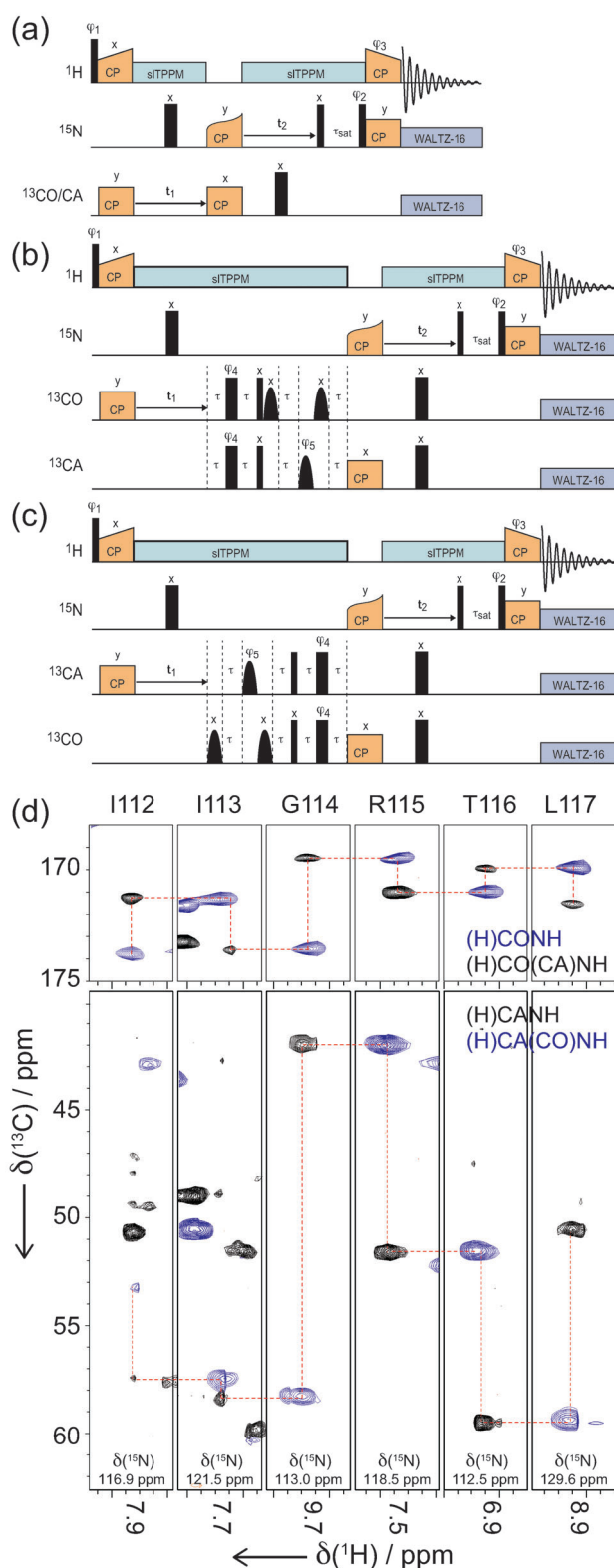
Figure 2. a–c) Pulse sequences used for proton-detected sequential assignment experiments. a) (H)CONH/(H)CANH; b) (H)CO(CA)NH; c) (H)CA(CO)NH. Narrow and broad black rectangles indicate 90^\circ and 180^\circ pulses, respectively, the bell shapes represent band-selective \pi -pulses, and the delay \tau is set to 1/4J (4.7 ms for J_{\text{COCA}} = 53 Hz). More details are available in the Supporting Information. d) Representative strips from proton-detected assignment of human [100% ^1\text{H} , ^2\text{H} , ^{13}\text{C} , ^{15}\text{N} ]-Zn II -SOD at 1 GHz and 60 kHz MAS: (H)CONH, (H)CO(CA)NH (blue and black contours of the upper plot, respectively), (H)CANH, (H)CA(CO)NH (black and blue contours of the lower plot, respectively). Sequential correlations are marked by the red line.
